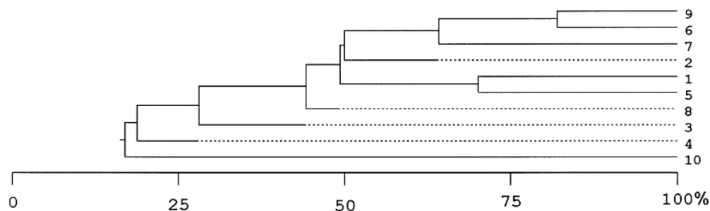
Figure 1. Dendrogram obtained by cluster analysis on the initial data... TNR 11, Center
